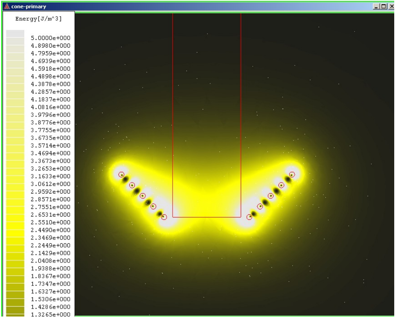
Magnified energy
