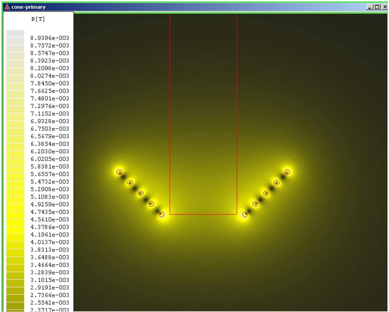
B Field
