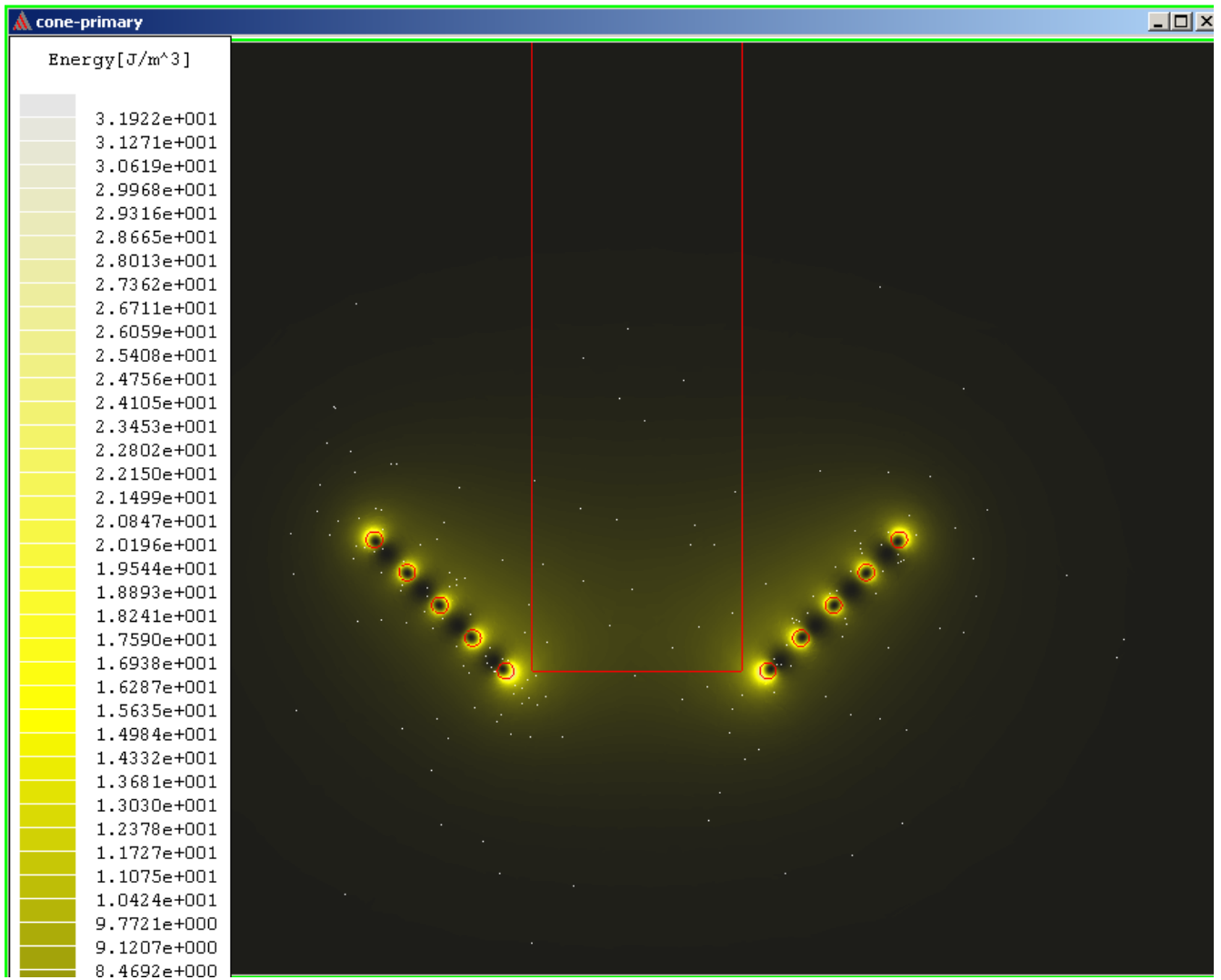
Energy (J/m 3 )
