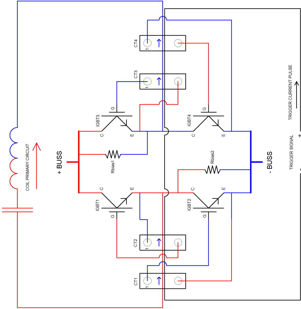
SYSTEM 1ST HALF CYCLE FORWARD CURRENT DRIVE
