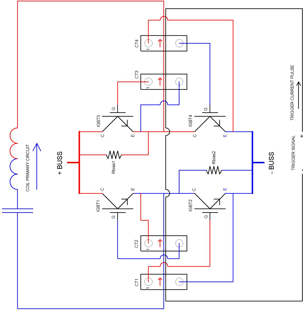
SYSTEM 1ST HALF CYCLE REVERSE CURRENT DRIVE
