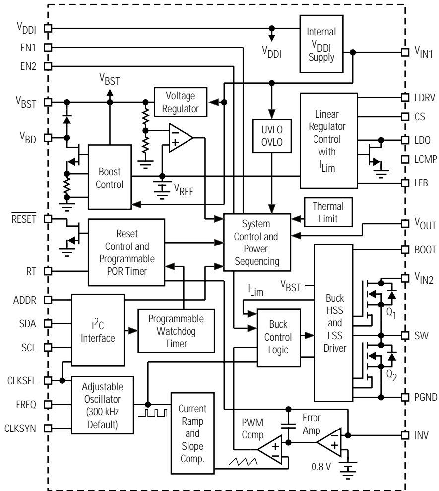
33702 Internal Block Diagram
