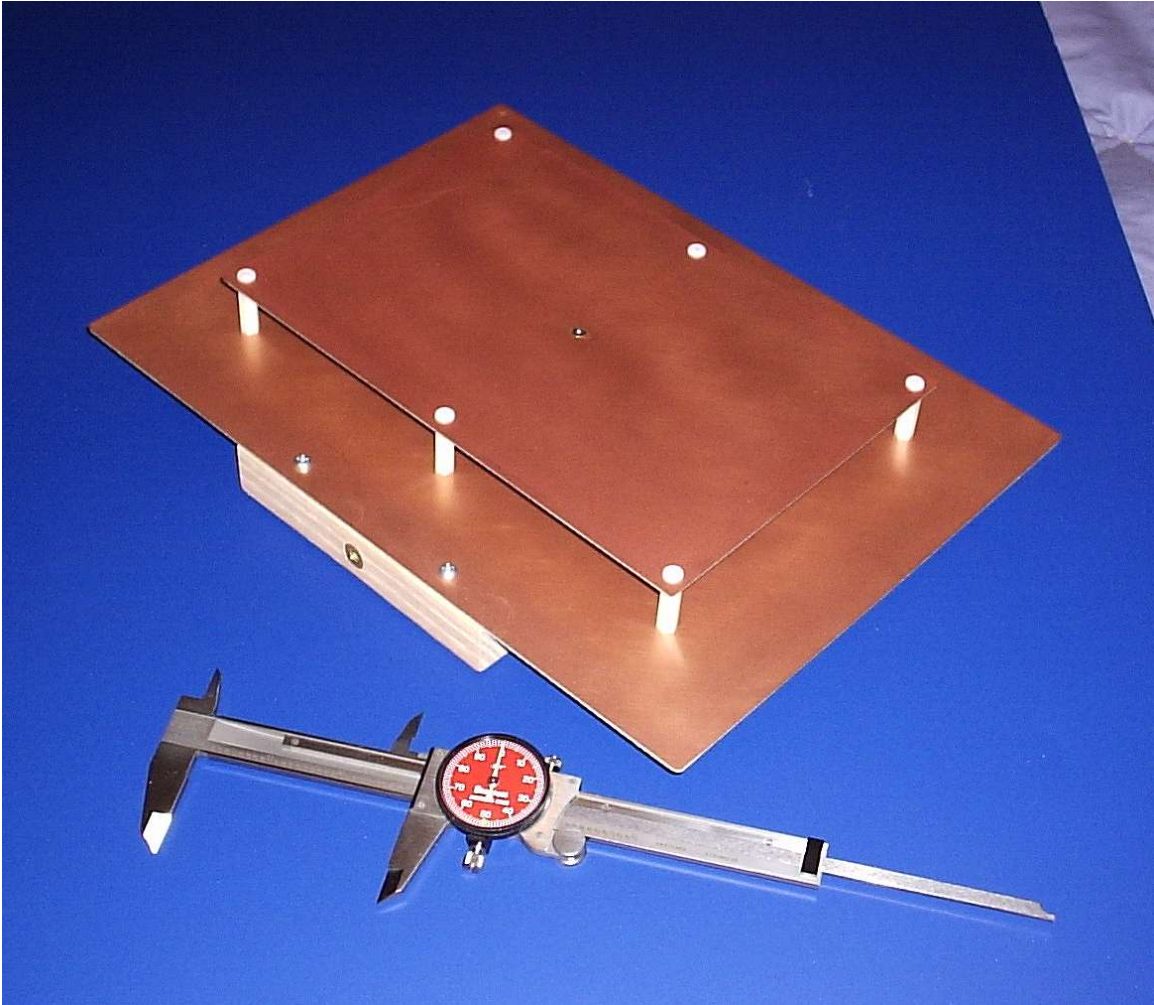
Two pieces of common single sided PCB material. 12 x 9 inches and 9 x 6 inches. Spaced with 1 inch 6-32 nylon spacers.
