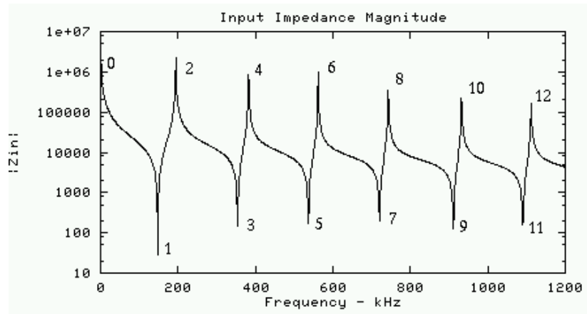
FIGURE 5.1. The input impedance spectrum
