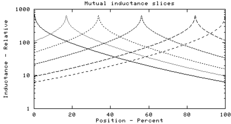
FIGURE 3.1. Typical mutual inductance distribution
