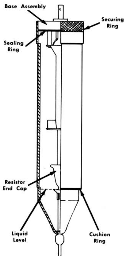
PROBE BODY
